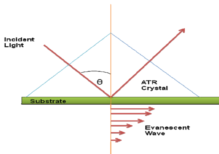
Figure 1. Evanescent wave
