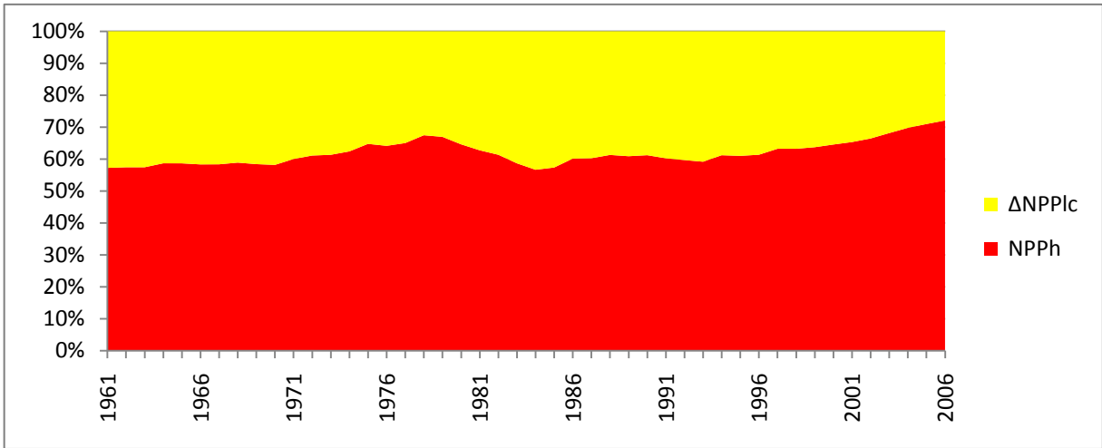
Figure 22: aNPP h and ΔaNPP lc as percentage of aHANPP
