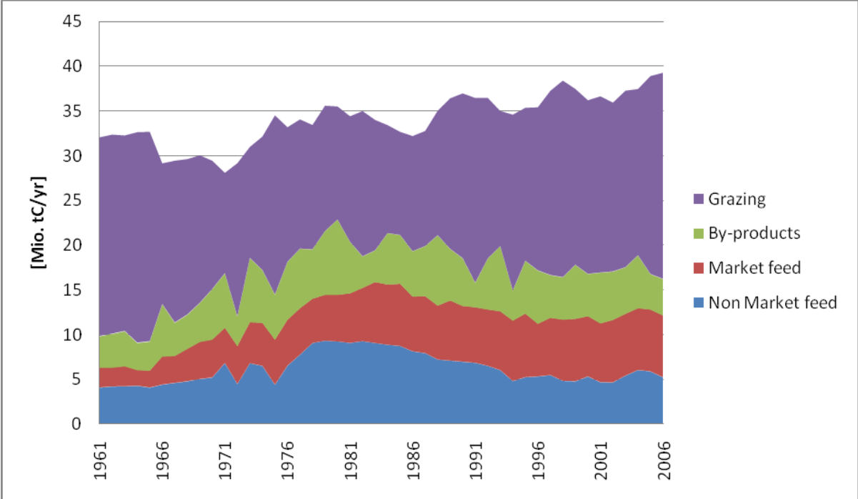
Figure 18: Feed supply for livestock species from 1961 to 2006
