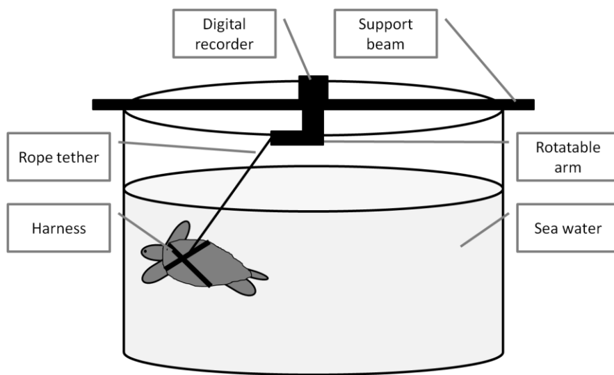
Figure 1. Circular experimental arena, commonly used to test sea turtle swimming orientations, including a turtle wearing a harness which is attached to a rotatable arm and a digital recorder.
