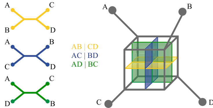
Figure 1.2. The information from all alternative tree topologies for species A, B, C, D (yellow, blue and green trees) can be displayed on one split network (right panel). We denote a bipartition of species by a vertical bar “|”. The central edges on the trees define incompatible bipartitions AB|CD , AC|BD , and AD|BC , while the remaining trivial bipartitions are common for all trees: A|BCD , B|ACD , C|ABD , and D|ABC . The split network combines all bipartitions from these trees. By cutting along planes inside the cube of a network one retrieves back three incongruent splits. The trivial splits, separating one species from the rest, are obtained from the network by cutting edges incident to species A, B, C, D .
