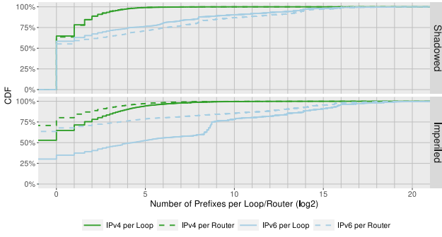
Fig. 9. Most loops (IPv4: 64.70%, IPv6: 58.43%) resp. routers (IPv4: 63.57%, IPv6: 55.19%) shadow only a single prefix. Only 29.23% (IPv4) resp. 36.46% (IPv6) of the routers, that are involved in loops, imperil other prefixes.
