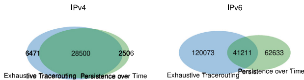
Fig. 7. 81.50% (28,500/34,971) of the IPv4 loop candidates were found again in the persistence measurements; for IPv6, this holds for only 25.55% (41,211/161,284).
