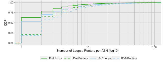
Fig. 16. Most AS are involved in a single loops (62.92%/53.42%), and operated two routers involved in loops (45.07%/38.72%).
