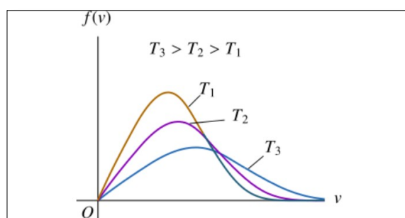
Figure 1 Maxwell-Boltzmann distribution of molecular speeds.
