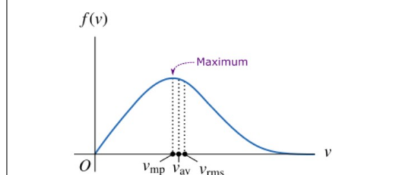
Figure 2 Most probable, average and root-mean-square speed.
