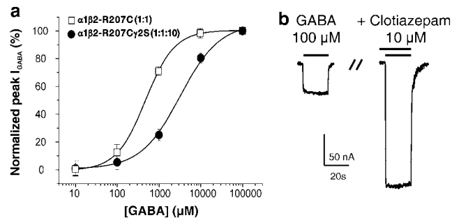
Figure 5 (a) GABA concentration–response curves of oocytes expressing \alpha 1\beta 2\text{-R207C} (1:1, EC_{50} = 486 \pm 81 \mu\text{M} , \eta_H = 1.2 \pm 0.2 , n = 6 ) and \alpha 1\beta 2\text{-R207C}\gamma 2S (1:1:10, EC_{50} = 3217 \pm 378 \mu\text{M} , \eta_H = 0.9 \pm 0.1 , n = 18 ) receptors. (b) Representative traces for enhancement of I_{GABA} through \alpha 1\beta 2\text{-R207C}\gamma 2S . Control currents (GABA) in the absence of clotiazepam and corresponding currents elicited by co-application of GABA and clotiazepam are shown.
