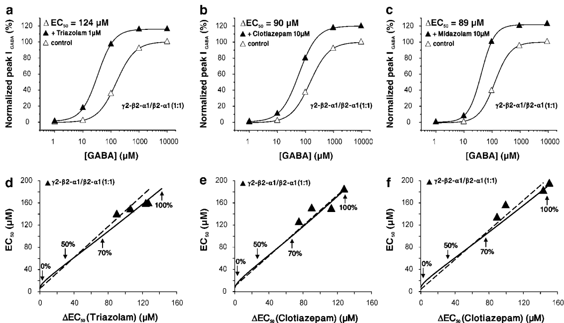
Figure 4 GABA concentration–response curves of oocytes injected with concatenated subunits ( \gamma 2\text{-}\beta 2\text{-}\alpha 1/\beta 2\text{-}\alpha 1 ) in the absence (control) and presence of 1 \mu\text{M} triazolam (a), 10 \mu\text{M} clotiazepam (b) and 10 \mu\text{M} midazolam (c). The corresponding EC_{50} values were: 158 \mu\text{M} (control), 34 \mu\text{M} (triazolam); 150 \mu\text{M} (control), 60 \mu\text{M} (clotiazepam); 132 \mu\text{M} (control), 43 \mu\text{M} (midazolam). EC_{50} values of the GABA concentration–response curves of oocytes expressing concatenated subunit constructs ( \gamma 2\text{-}\beta 2\text{-}\alpha 1 and \beta 2\text{-}\alpha 1 in 1:1 ratio) and \Delta EC_{50} (BZD)s induced by (d) 1 \mu\text{M} triazolam, (e) 10 \mu\text{M} clotiazepam and (f) 10 \mu\text{M} midazolam were added to the regression lines from Figures 2d–f. Corresponding regression lines (dashed) were taken from Figures 2d–f and extended towards the values of the concatenated subunits. Solid lines (d–f) represent the non-linear fit of Equations 1–5 (see Materials and methods) by the maximal likelihood. Calculated current fractions of \gamma -incorporating receptors (0, 50, 70 and 100%) are indicated. Each graph (a, b and c) and each data point (d, e and f) represent one experiment on one oocyte.
