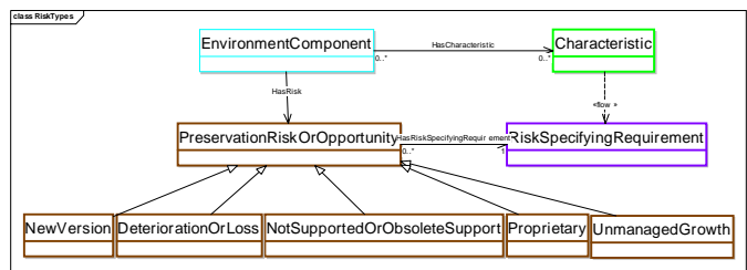
Figure 6 Risk Types
