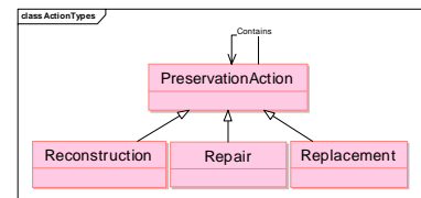
Figure 7 Action Types
