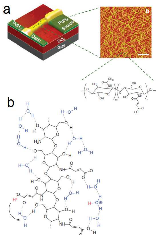
Fig. 4. a) Bioprotonic transistor based on chitosan as a proton-conducting material. b) Illustration of the Grotthus-like mechanism of proton conduction along the chitosan polysaccharide. Reproduced with permission from ref. 56.
