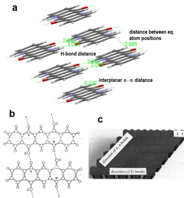
Fig. 8. a) Crystal packing in \beta -quinacridone, which consists of infinite linear chains of H-bonded molecules. b) quinacridone H-bonding in the linear-chain polymorphs. c) Schematic illustration of the “bricks-in-a-wall” crystal packing present in many H-bonded pigments, whereby linear chains of H-bonding propagate along one direction, while there is \pi - \pi stacking perpendicular to the H-bonding direction. Reproduced with permission from ref. 71
