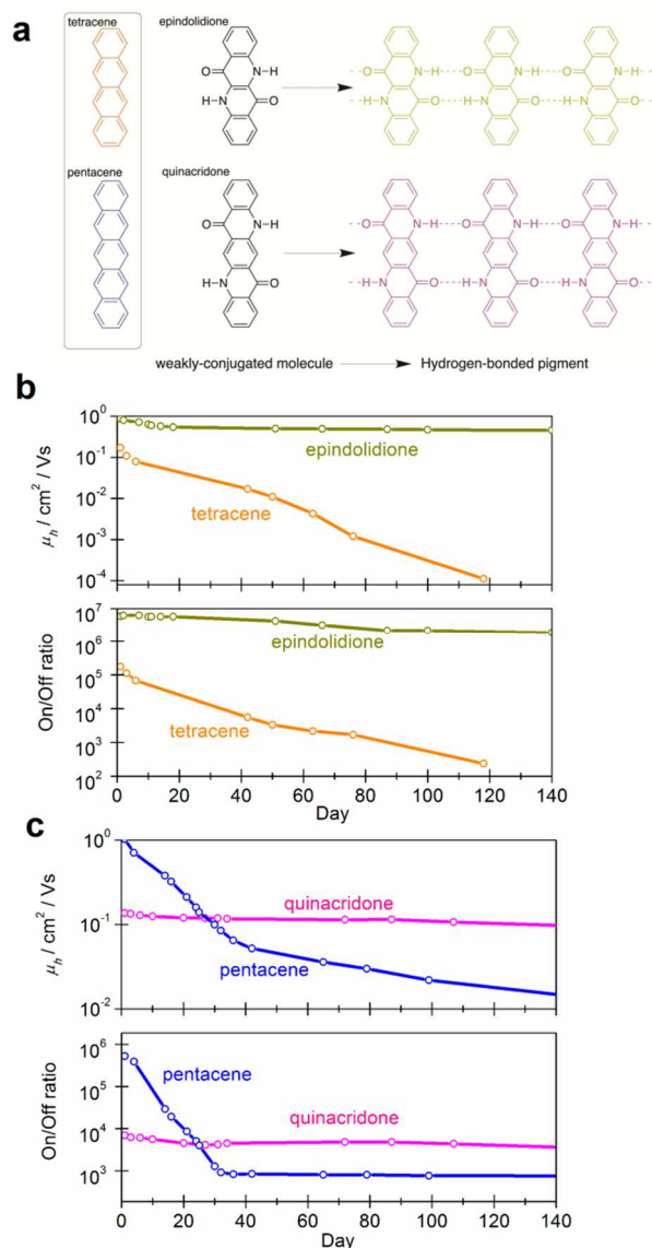
Fig. 7. a) The acenes and their structural H-bonded analogues, epindolidione and quinacridone, reported in Ref. 67 . b) Comparison of operational stability in air of tetracene and epindolidione. c) Comparison of operational stability in air of pentacene and quinacridone. Reproduced with permission from Ref. 67
