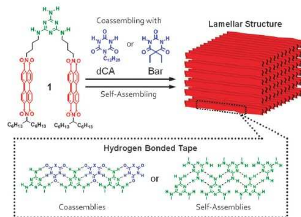
Fig. 10. Perylene bisimide conjugated dyes functionalized with melamine segments, providing self-assembly to yield H-bonded self-organized “tapes” allowing electron-transport through stacked perylene bisimide moieties. Reproduced with permission from Ref. 105
