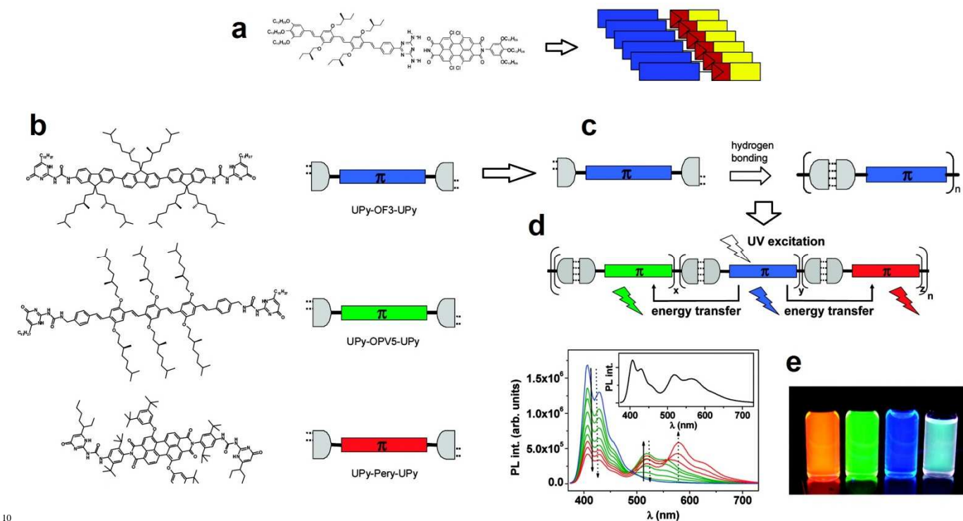
Fig. 9. a) Complementary H-bonded self-assembly of a hole-conducting conjugated molecule oligo(phenylenevinylene) and an electron-transporting one, perylene bisimide, resulting in an ambipolar-transporting supramolecular material, from Ref. 101 b) Blue, green, and red fluorophores functionalized with complementary H-bonding end groups. c) H-bonding mediated self-assembly of fluorophores, resulting in an efficient energy cascade to produce white light emission, d) and e). Reproduced with permission from Ref. 102
