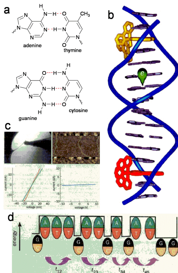
Fig. 2. a) DNA base pairs held together by complementary H-bonds. b) Experimental technique of Barton et al. whereby fluorescence quenching via charge transfer of dyes intercalated at different positions along a DNA strand is used to measure electronic conduction through the base pair stack. Reproduced with permission from ref. 28 c) Examples of contacting individual DNA strands for electrical measurements. These experiments yielded controversial results. Reproduced from ref. 27 d) Multiple researchers have concluded that conduction proceeds through stacked G-C pairs, however A-T pairs are a barrier. From ref. 27
