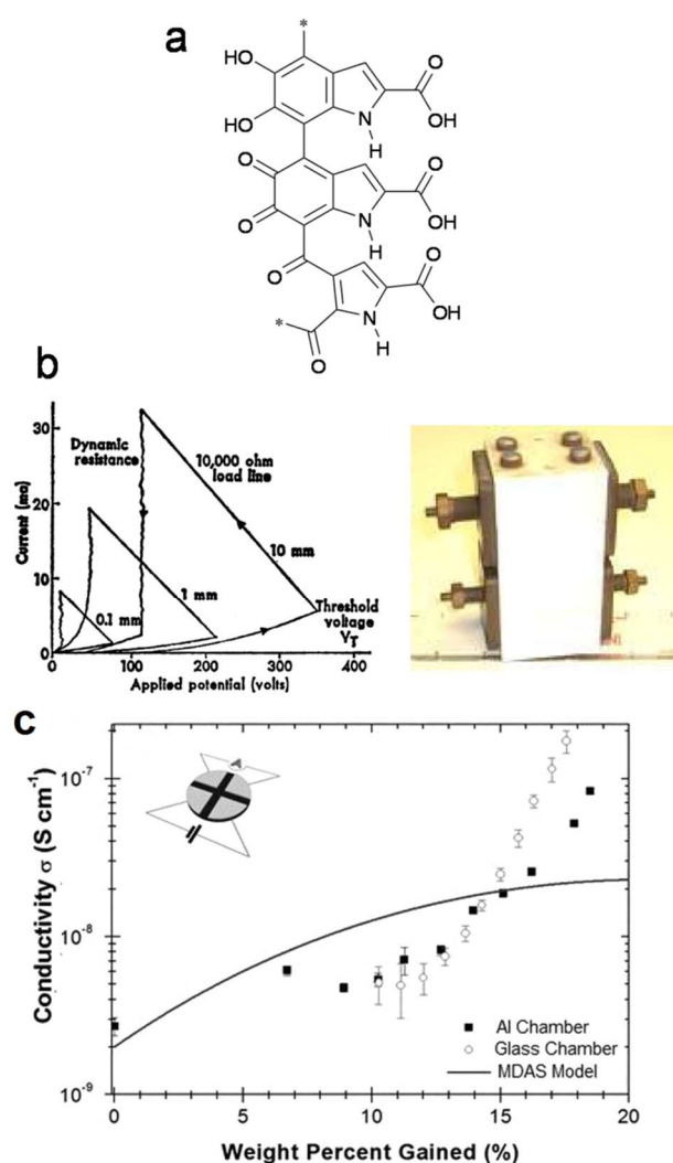
Fig. 3. a) An example of the polymerized heterocycles that comprise melanin. b) I-V characteristics and photograph of the original melanin “threshold switch” device fabricated by McGinness. c) Relationship of conductivity to water uptake in melanin, from ref. 41
