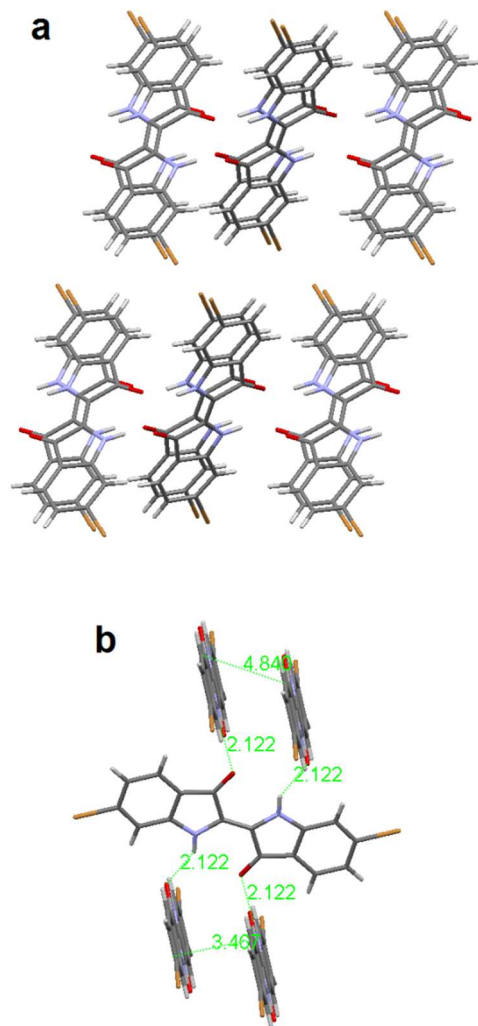
Fig. 6. a) View down the b-axis, or \pi -stacking axis, of tyrian purple. b) Crystal packing in tyrian purple, showing the interplanar, atom-to-atom, and H-bond distances. Each molecule is H-bonded to 4 neighbours.
