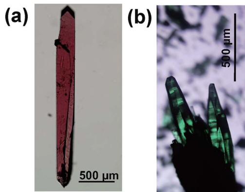
Fig. 1 Single crystals of (a) \text{CoAs}_2\text{O}_4 and (b) \text{NiAs}_2\text{O}_4 .
