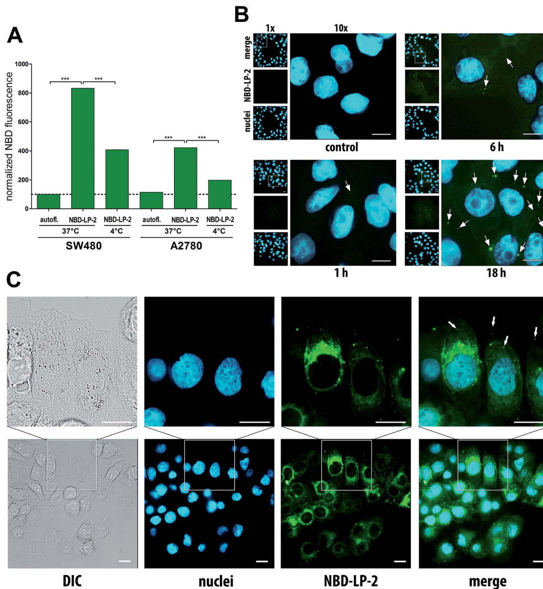
Fig. 5 Cellular uptake of fluorescence (NBD)-labeled LP-2. (A) SW480 and A2780 cells were treated with NBD-LP-2 (8 \mu\text{M} referred to NBD) for 1 h at 37 ^{\circ}\text{C} or 4 ^{\circ}\text{C} , washed once with PBS and analyzed by flow cytometry for fluorescence intensity. *** p < 0.001 one-way ANOVA with Bonferroni posttest. (B) Fluorescence microscopy of time-dependent liposome uptake in SW480 cells treated with NBD-LP-2 (33 \mu\text{M} referred to NBD) for 1, 6 and 18 h at 37 ^{\circ}\text{C} . (C) Fluorescence microscopy of long-term liposomal uptake in SW480 cells after treatment with NBD-LP-2 (33 \mu\text{M} ) for 24 h at 37 ^{\circ}\text{C} . After fixation with 4% paraformaldehyde, nuclei were stained with DAPI. Micrographs were taken with a fluorescence microscope in differential interference contrast (DIC), green (liposomes) and UV (nuclei) channels. Size bar = 20 \mu\text{m} .
